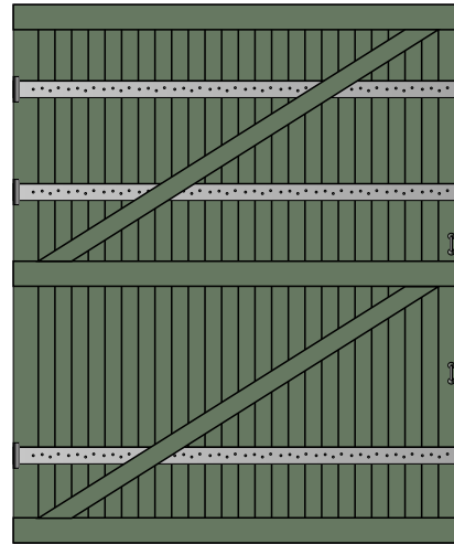
Rear door covering
