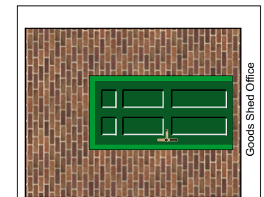
Goods Shed Right Outer Wall - 2mm Card
