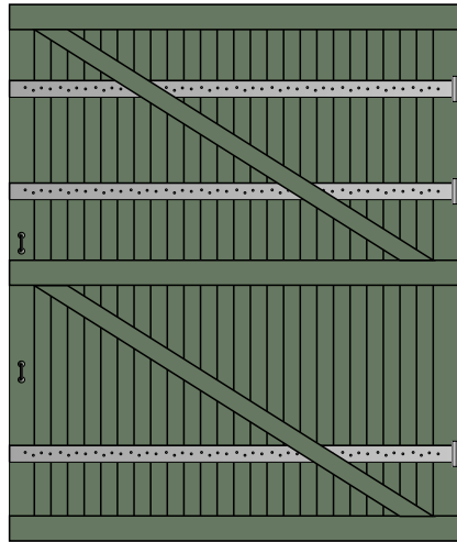
Front door covering
